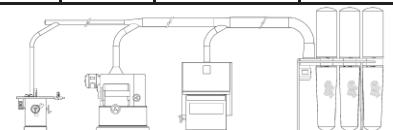
Diagram of DUSTEK Model C750 dust collector installation connected to a 10" tilting arbor saw table, a 24" single surface planer, and a 36" conveyor feed wide belt sander.
